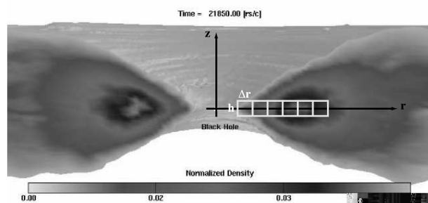
Fig. 1. A perspective view of 3-D MHD accretion flows. Gray-scale indicates the normalized density. A black hole is located at the origin.
