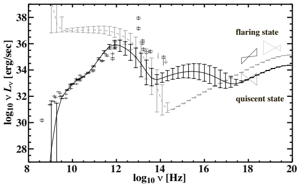
Fig. 5. Spectral Energy Distribution (SED) of MHD accretion flows ranging from radio to gamma-ray. Solid and dashed lines indicate the emergent spectra and the emitted spectra, respectively. Bars indicate the time variation. Cross points and “bow ties” indicate the observed spectra in the Galactic center (Narayan et al. 1998; Eckart et al. 2006; Baganoff 2001; Belandger et al. 2005)
