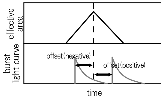
Fig. 2. A schematic picture of the definition of the offset time.
