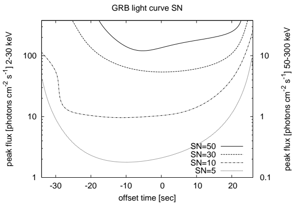
Fig. 4. The contour map of light curve S/N in the space of time offset of the burst and the flux of the burst. The horizontal axis is the offset time, which defined as shown in figure 2. The vertical axis is the flux of the burst. The contour of solid, dashed, dashed-dotted, and dotted line correspond to the S/N level of 50, 30, 10, and 5 respectively.
