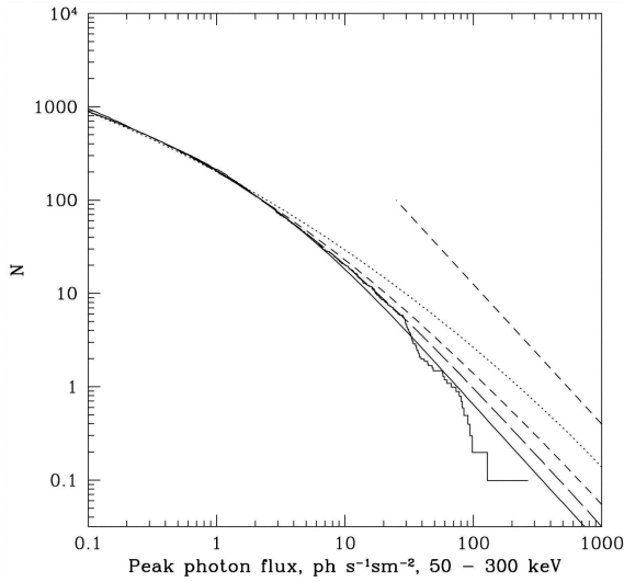
Fig. 5. The integral peak flux distribution of Ulysses/BATSE GRBs. This figure is from Stern et al. (2002).
