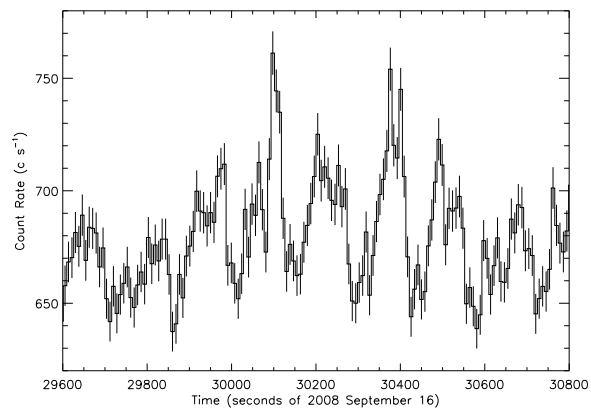
Fig. 8. An example of an accreting X-ray pulsar in the GBM data. This Figure shows 283-s pulses from Vela X-1 in the 12-52 keV energy band for GBM NaI 4.
