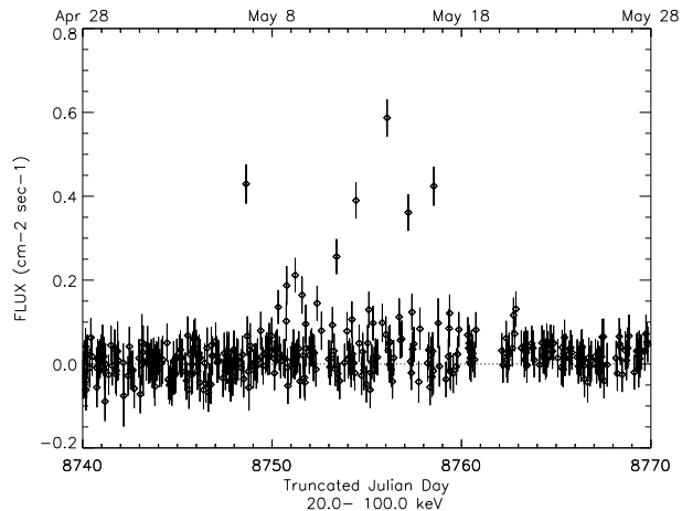
Fig. 3. From Paciasas et al. (1996). Single step Earth occultation measurements of GRS 1915+105 with BATSE in the 20-100 keV band during early May 1992. The high points on the plot are bright flares from GRS 1915+105 detected as large Earth occultation steps. For comparison, the flux from the Crab Nebula is \sim 0.3 \text{ ph cm}^{-2}\text{s}^{-1} in this band
